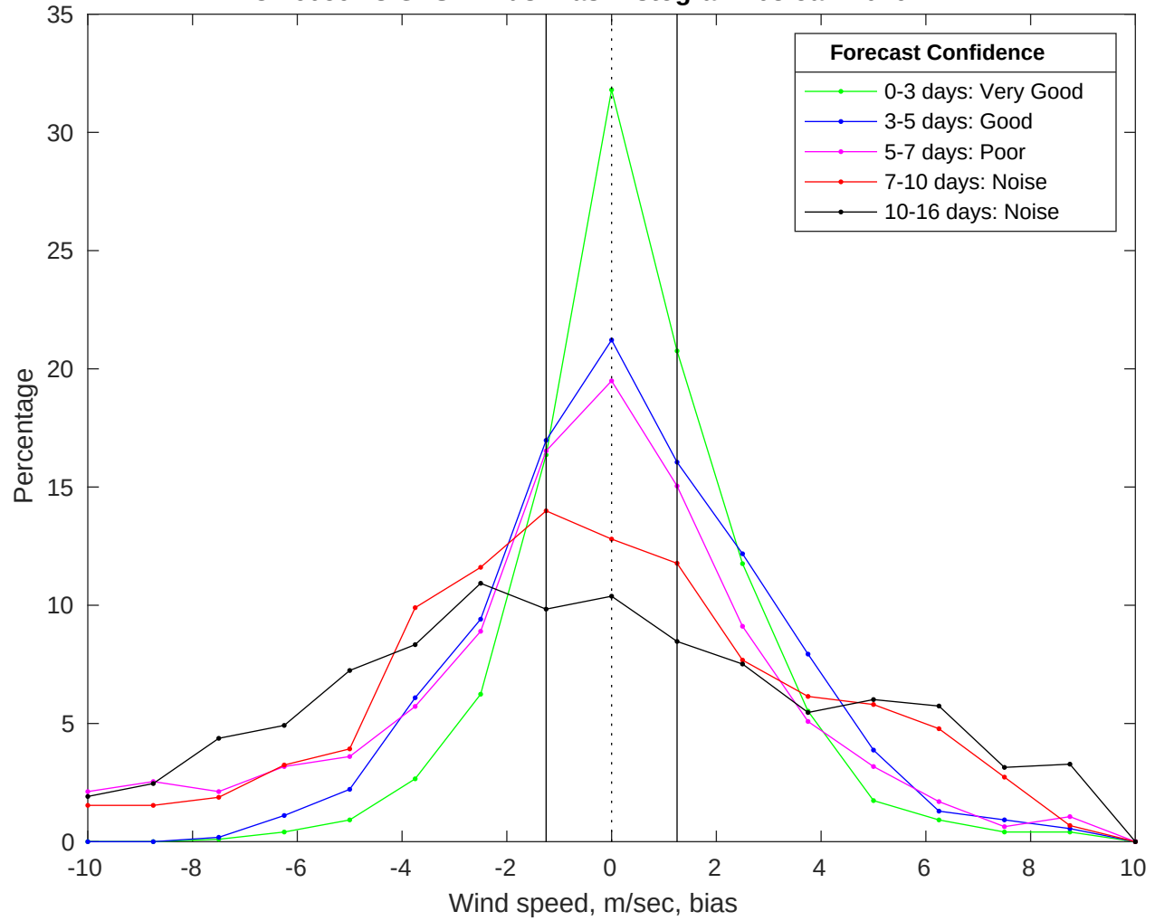
NDBC 46059 vs GFS Winds Bias Histogram: 08-Jan-2026
