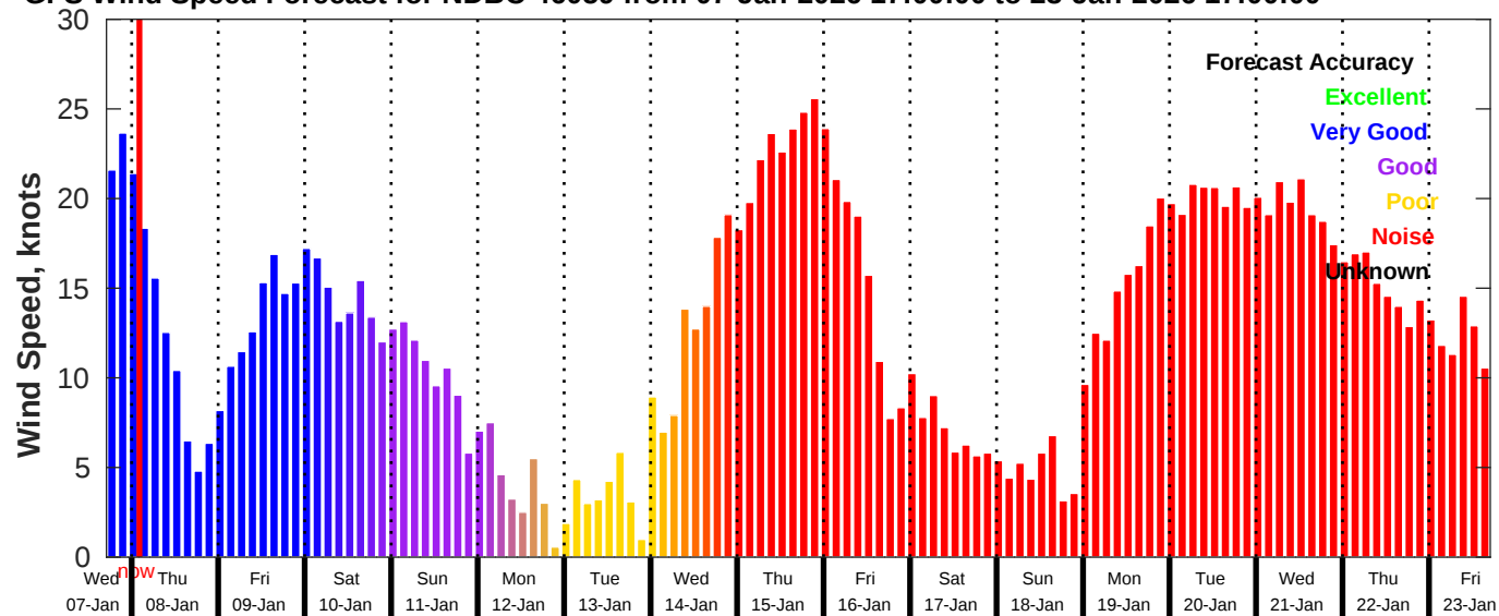
GFS Wind Speed Forecast for NDBC 46059 from 07-Jan-2026 17:00:00 to 23-Jan-2026 17:00:00
