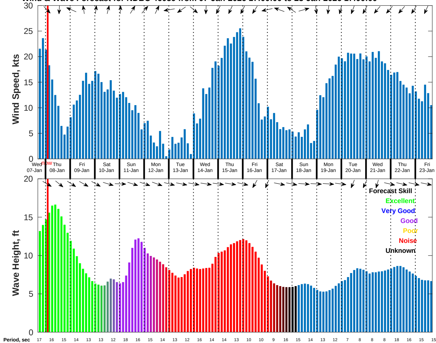
Wind & Wave Forecast for NDBC 46059 from 07-Jan-2026 17:00:00 to 23-Jan-2026 17:00:00
