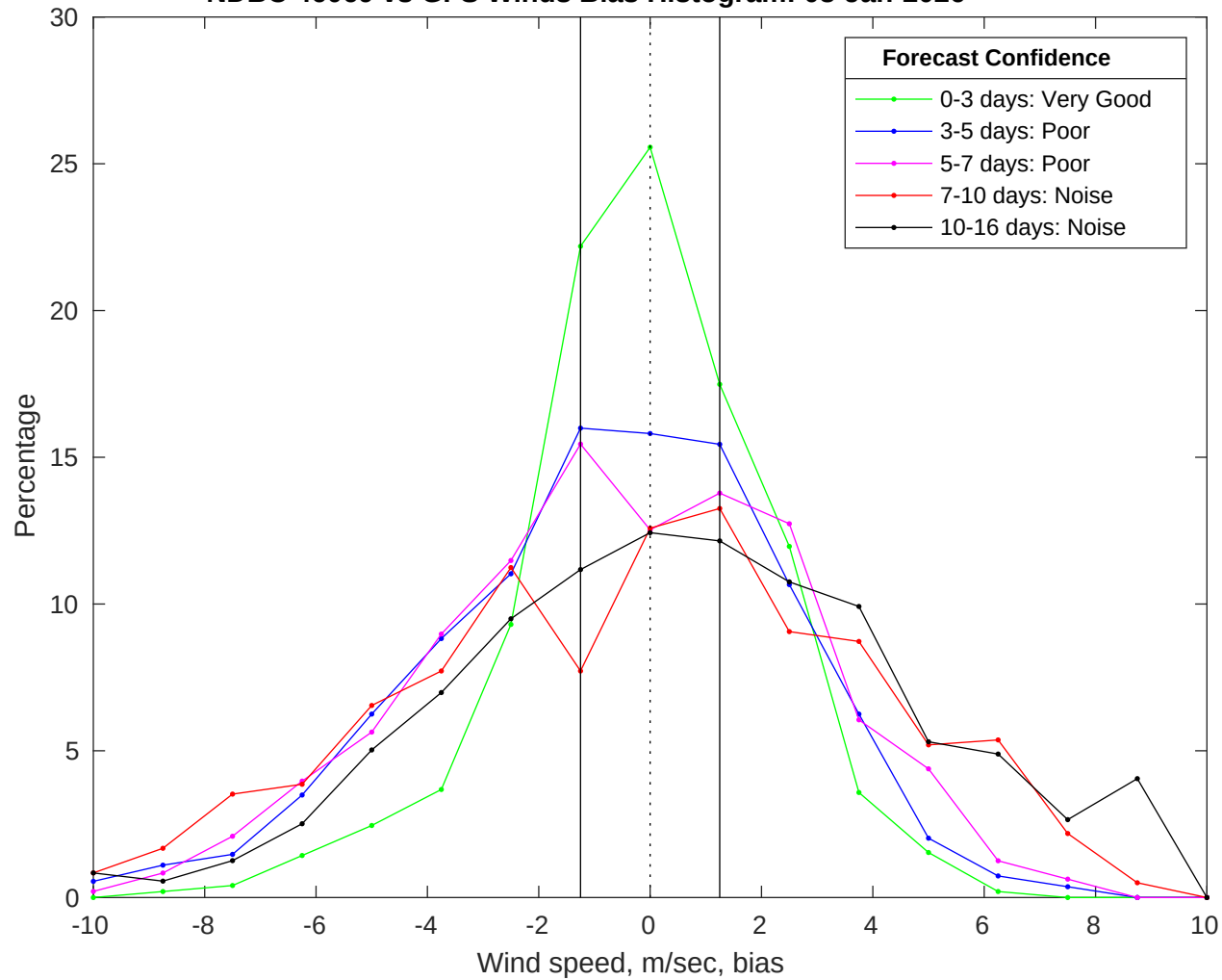
NDBC 46069 vs GFS Winds Bias Histogram: 08-Jan-2026
