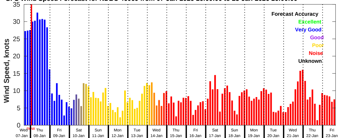
GFS Wind Speed Forecast for NDBC 46069 from 07-Jan-2026 16:00:00 to 23-Jan-2026 16:00:00
