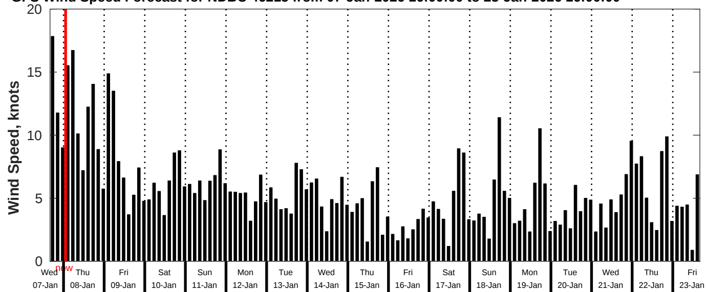
GFS Wind Speed Forecast for NDBC 46215 from 07-Jan-2026 16:00:00 to 23-Jan-2026 16:00:00
