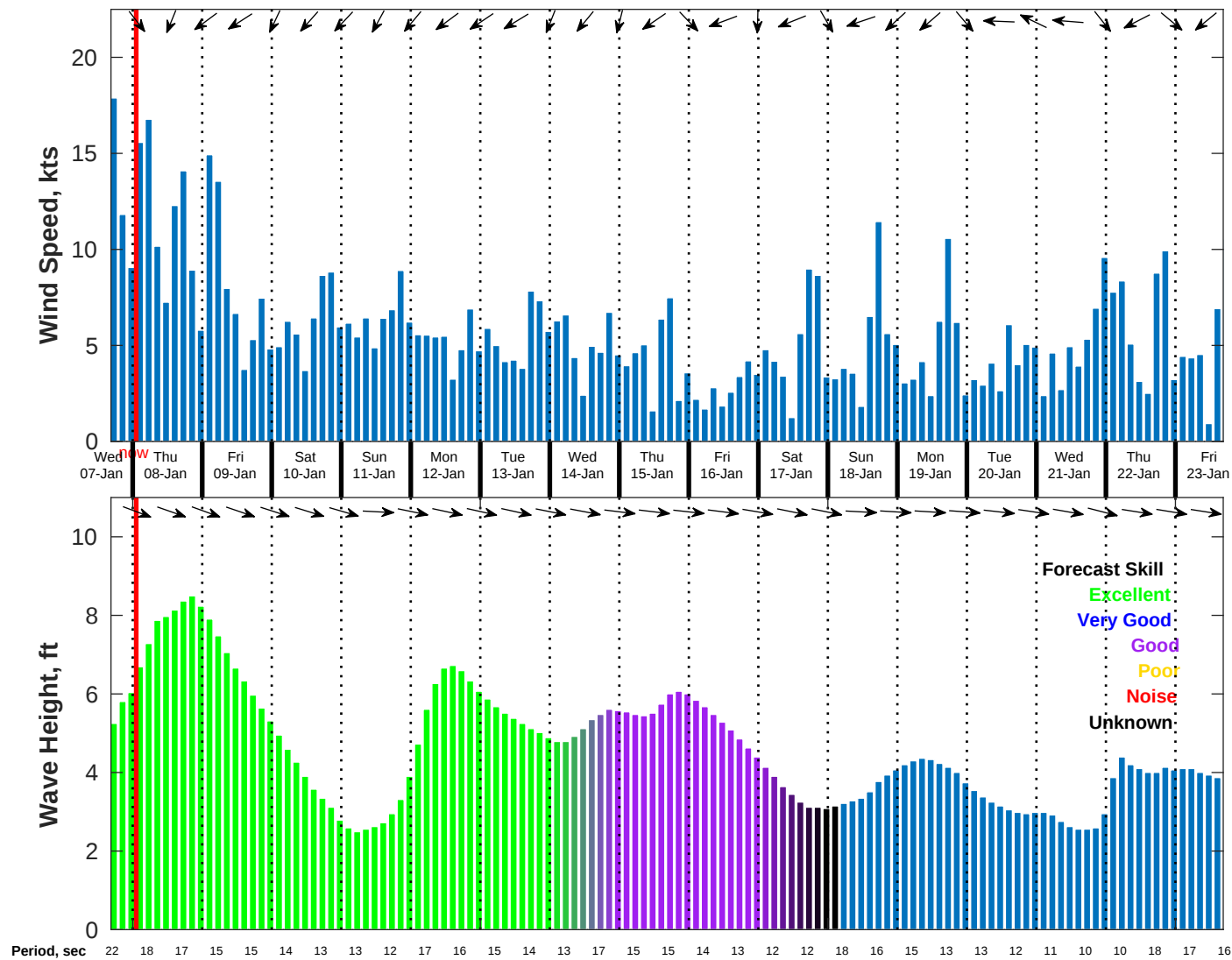
Wind & Wave Forecast for NDBC 46215 from 07-Jan-2026 16:00:00 to 23-Jan-2026 16:00:00
