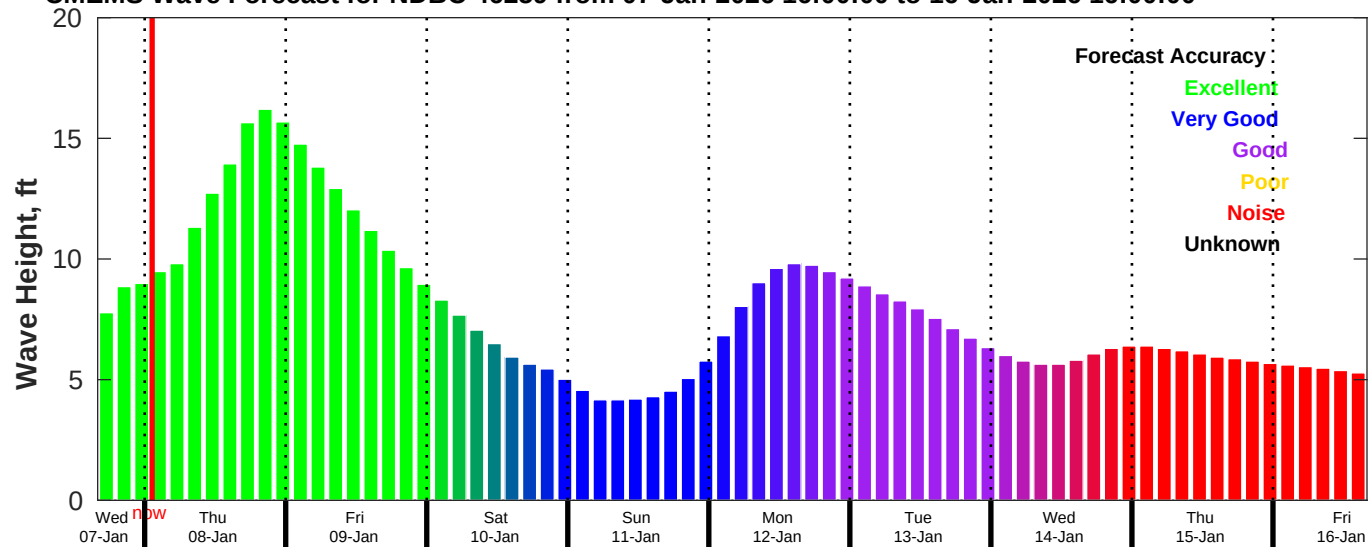
CMEMS Wave Forecast for NDBC 46259 from 07-Jan-2026 16:00:00 to 16-Jan-2026 16:00:00
