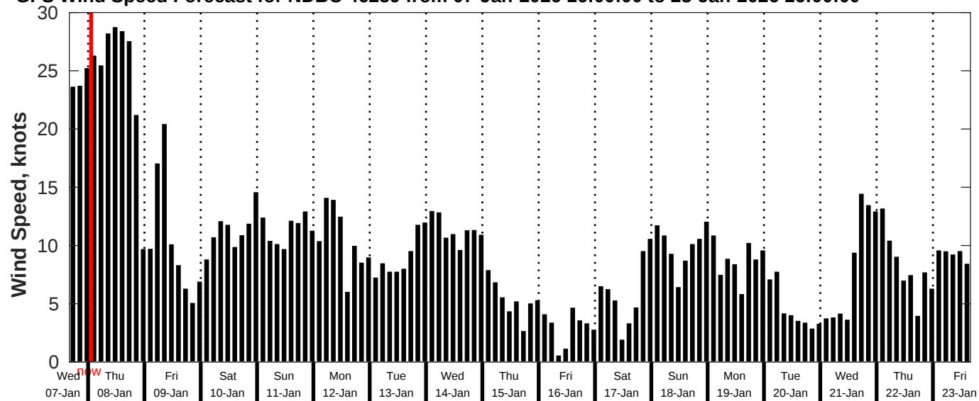
GFS Wind Speed Forecast for NDBC 46259 from 07-Jan-2026 16:00:00 to 23-Jan-2026 16:00:00
