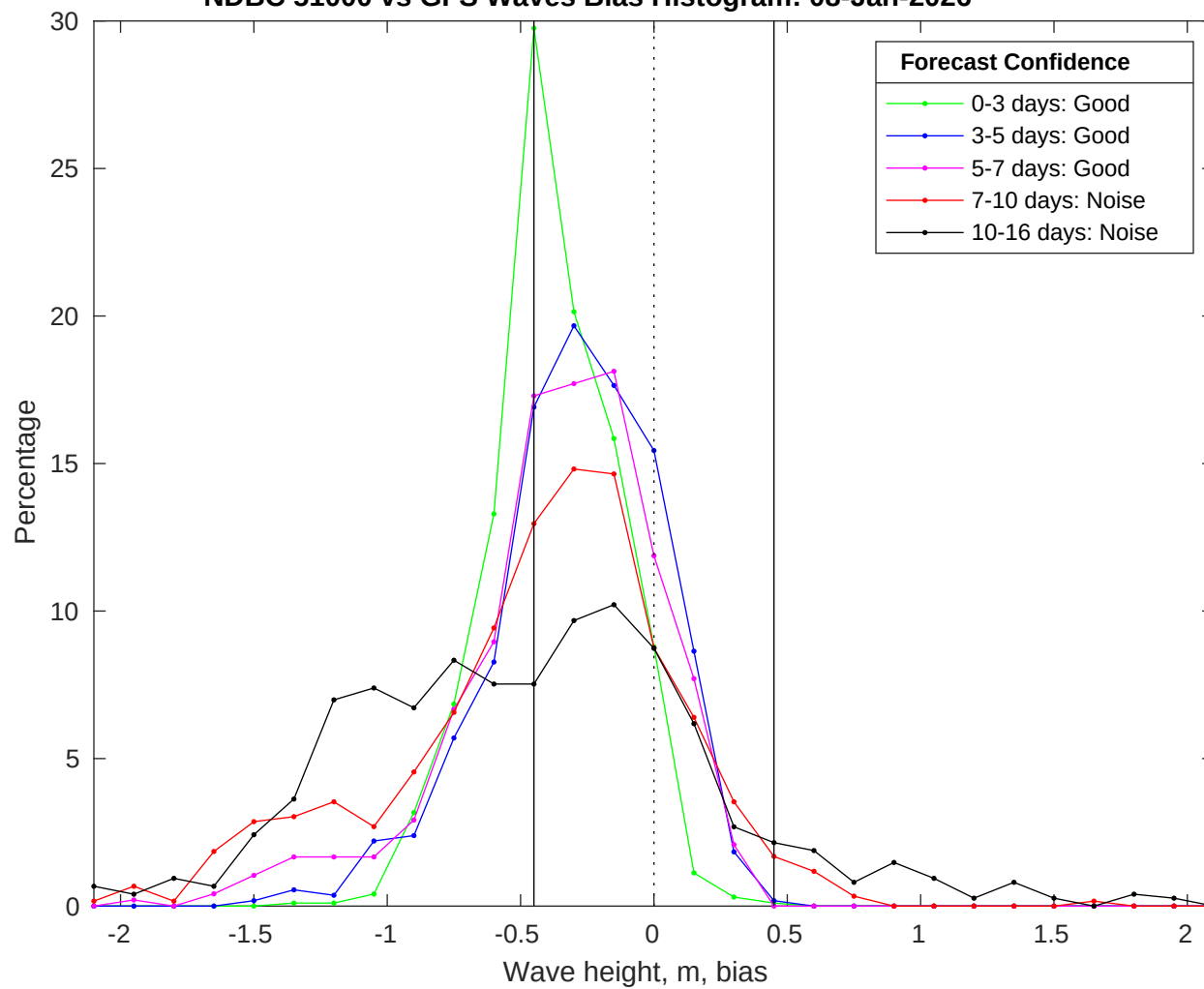
NDBC 51000 vs GFS Waves Bias Histogram: 08-Jan-2026
