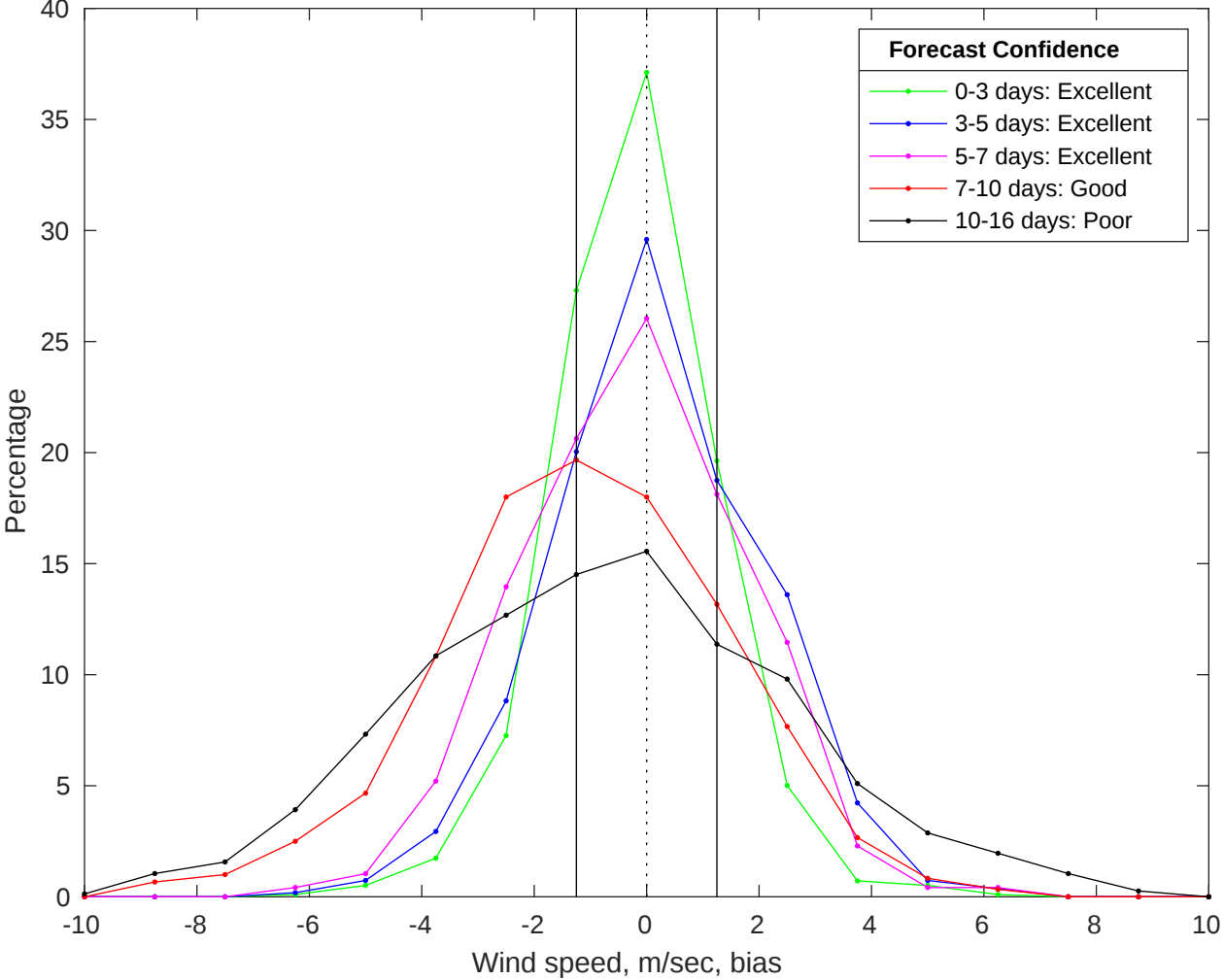
NDBC 51000 vs GFS Winds Bias Histogram: 08-Jan-2026
