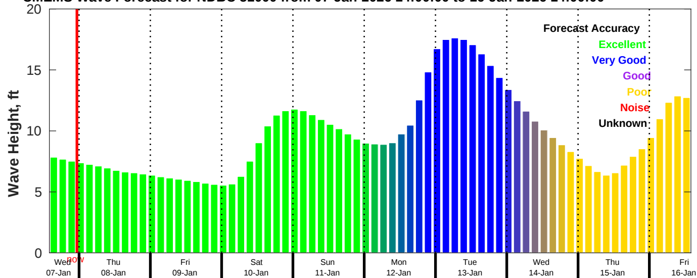
CMEMS Wave Forecast for NDBC 51000 from 07-Jan-2026 14:00:00 to 16-Jan-2026 14:00:00
