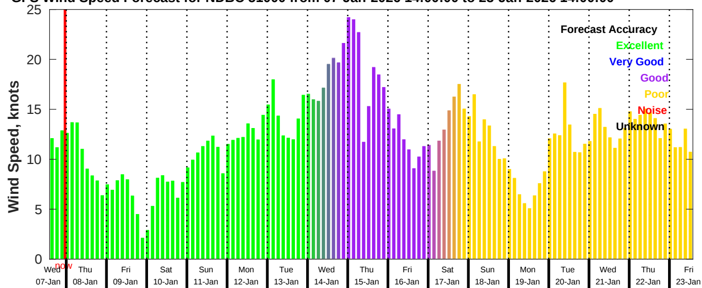
GFS Wind Speed Forecast for NDBC 51000 from 07-Jan-2026 14:00:00 to 23-Jan-2026 14:00:00
