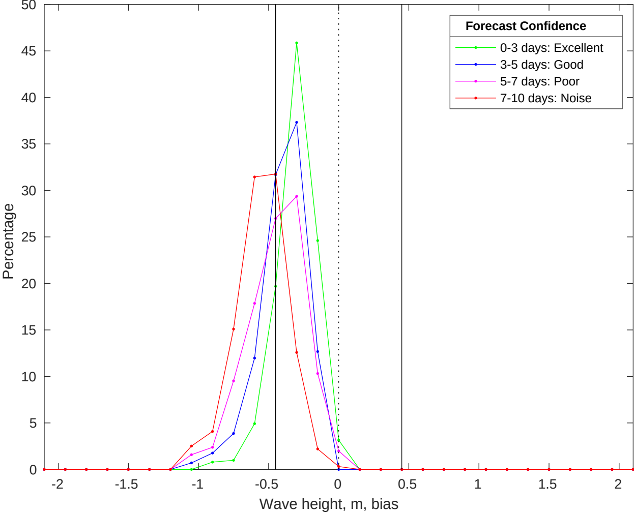
NDBC 51209 vs CMEMS Waves Bias Histogram: 08-Jan-2026
