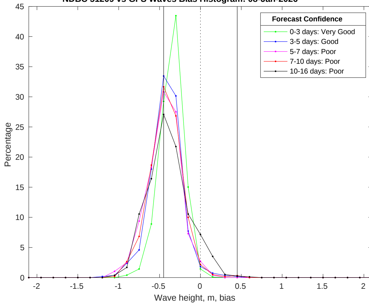
NDBC 51209 vs GFS Waves Bias Histogram: 08-Jan-2026
