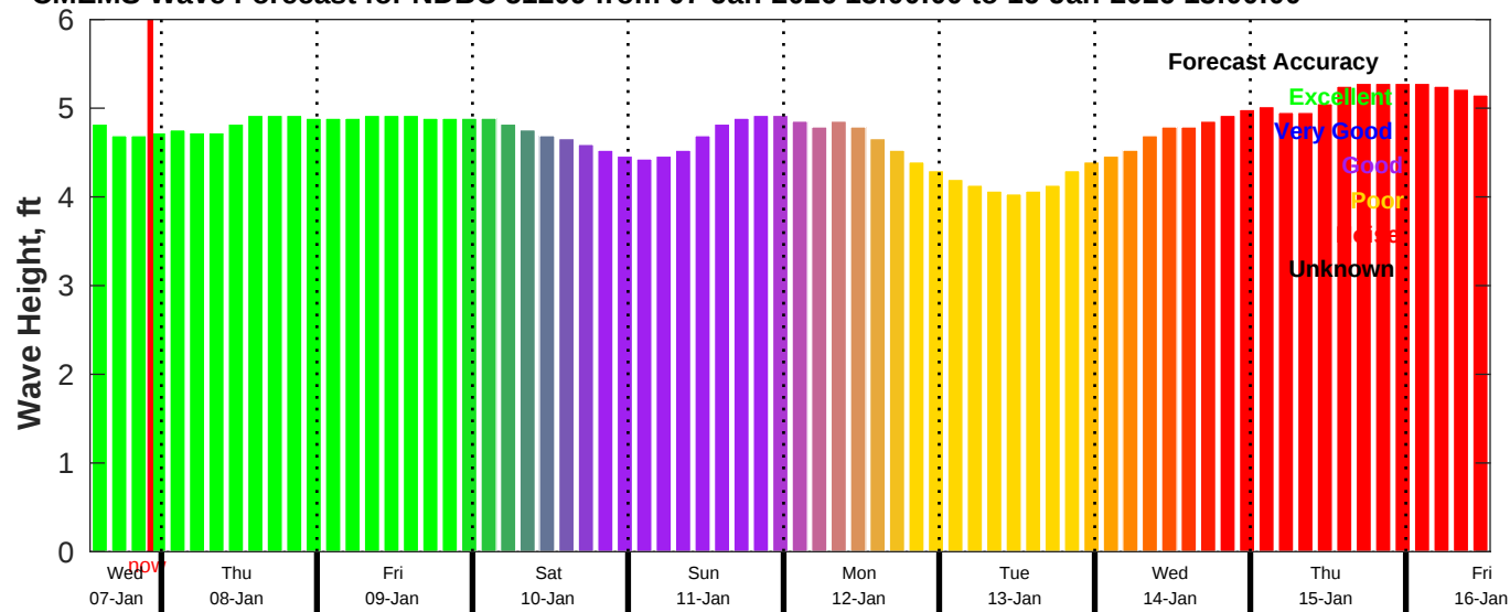
CMEMS Wave Forecast for NDBC 51209 from 07-Jan-2026 13:00:00 to 16-Jan-2026 13:00:00
