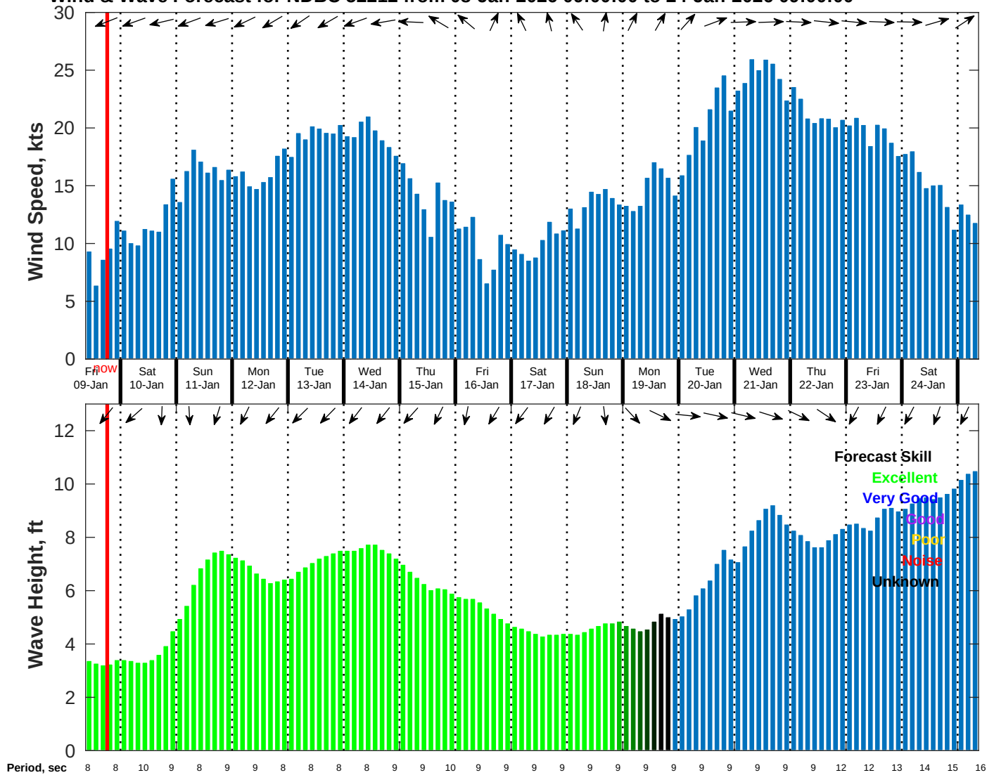
Wind & Wave Forecast for NDBC 52212 from 08-Jan-2026 09:00:00 to 24-Jan-2026 09:00:00
