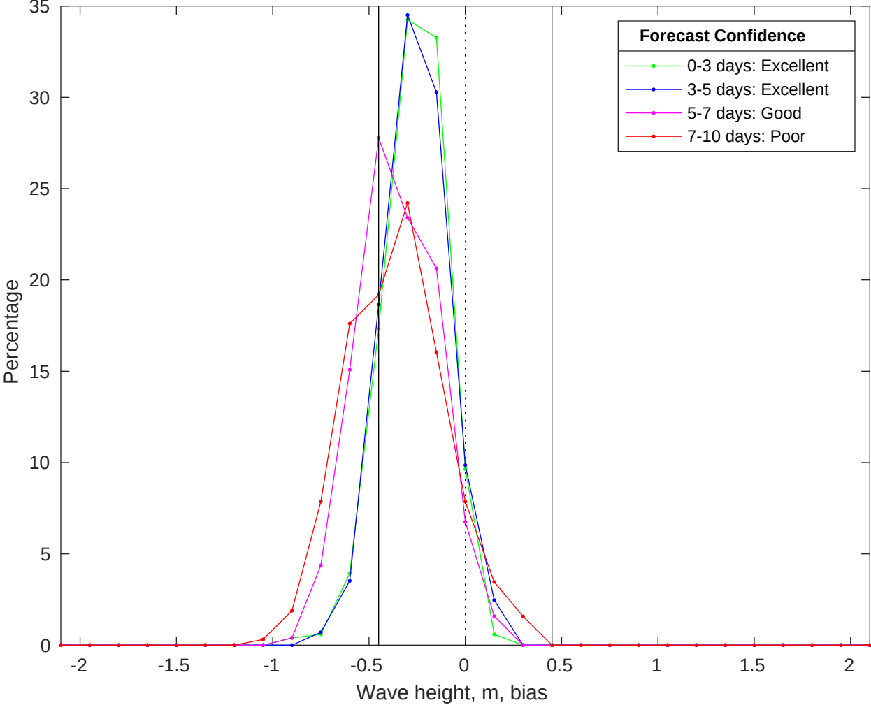
NDBC 52213 vs CMEMS Waves Bias Histogram: 08-Jan-2026
