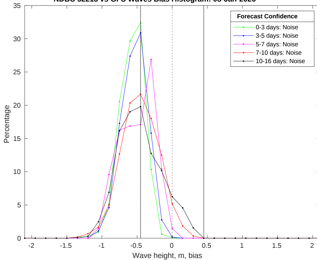
NDBC 52213 vs GFS Waves Bias Histogram: 08-Jan-2026
