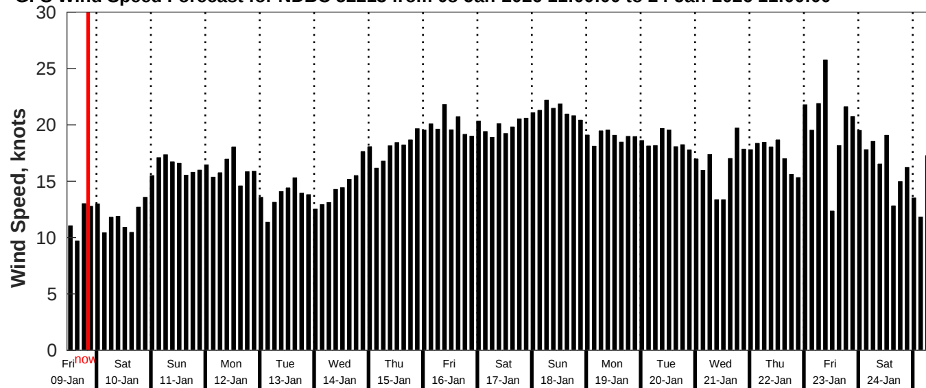
GFS Wind Speed Forecast for NDBC 52213 from 08-Jan-2026 11:00:00 to 24-Jan-2026 11:00:00
