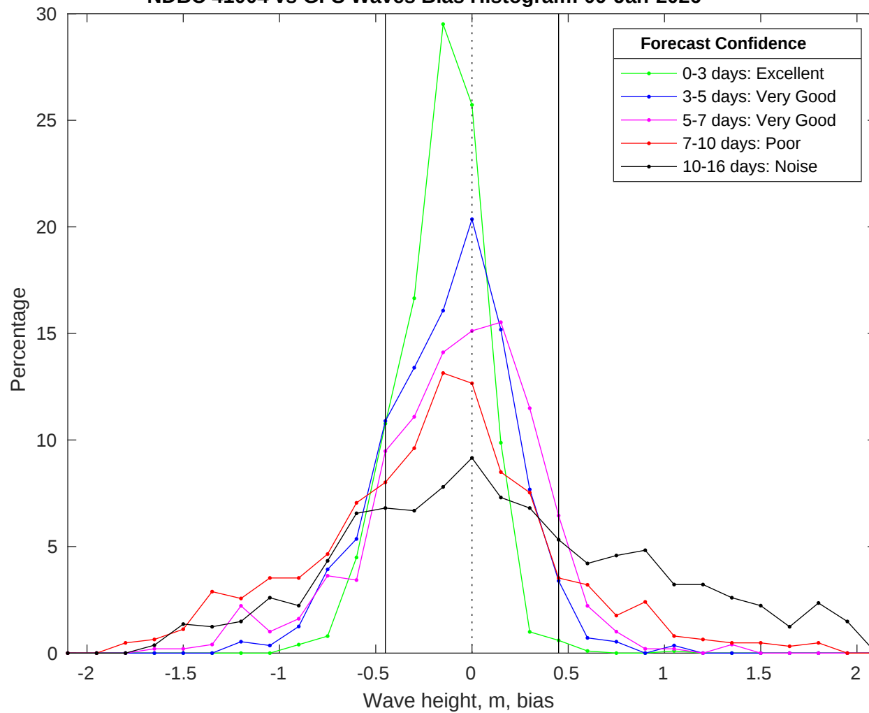
NDBC 41004 vs GFS Waves Bias Histogram: 09-Jan-2026
