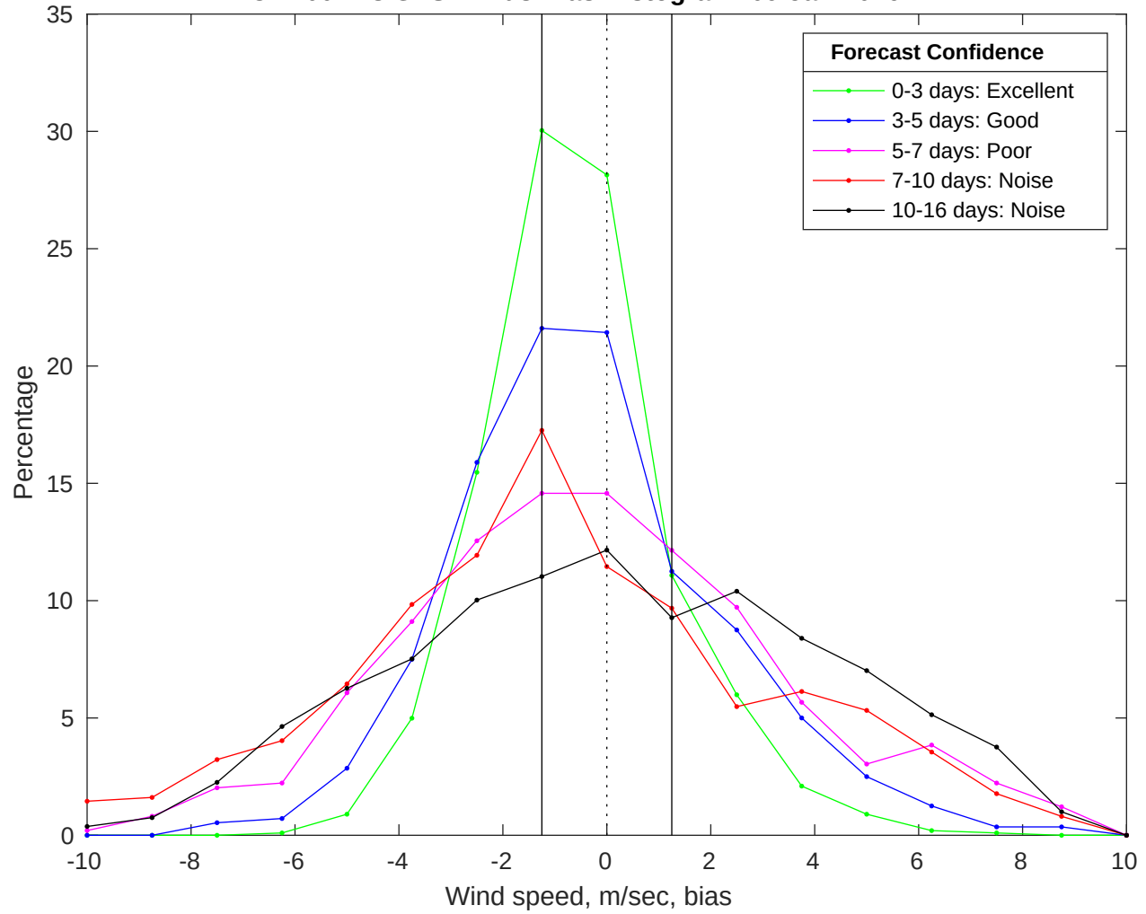
NDBC 41004 vs GFS Winds Bias Histogram: 09-Jan-2026
