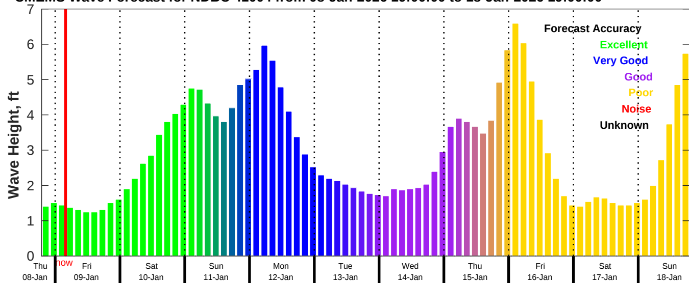
CMEMS Wave Forecast for NDBC 41004 from 08-Jan-2026 19:00:00 to 18-Jan-2026 19:00:00
