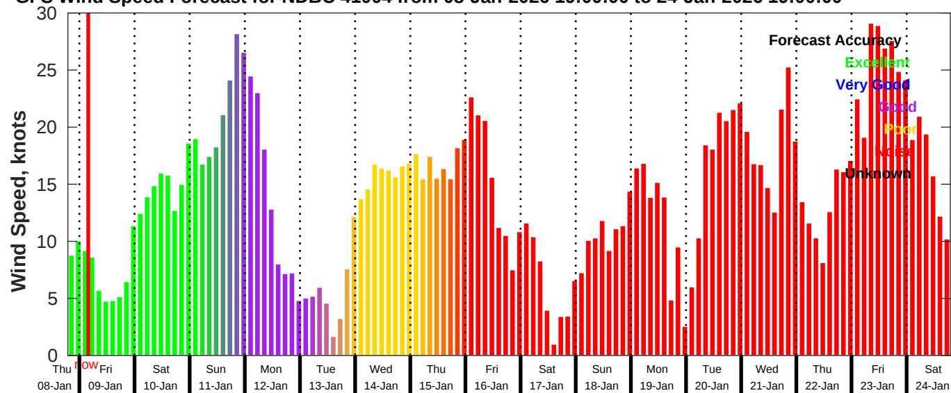
GFS Wind Speed Forecast for NDBC 41004 from 08-Jan-2026 19:00:00 to 24-Jan-2026 19:00:00
