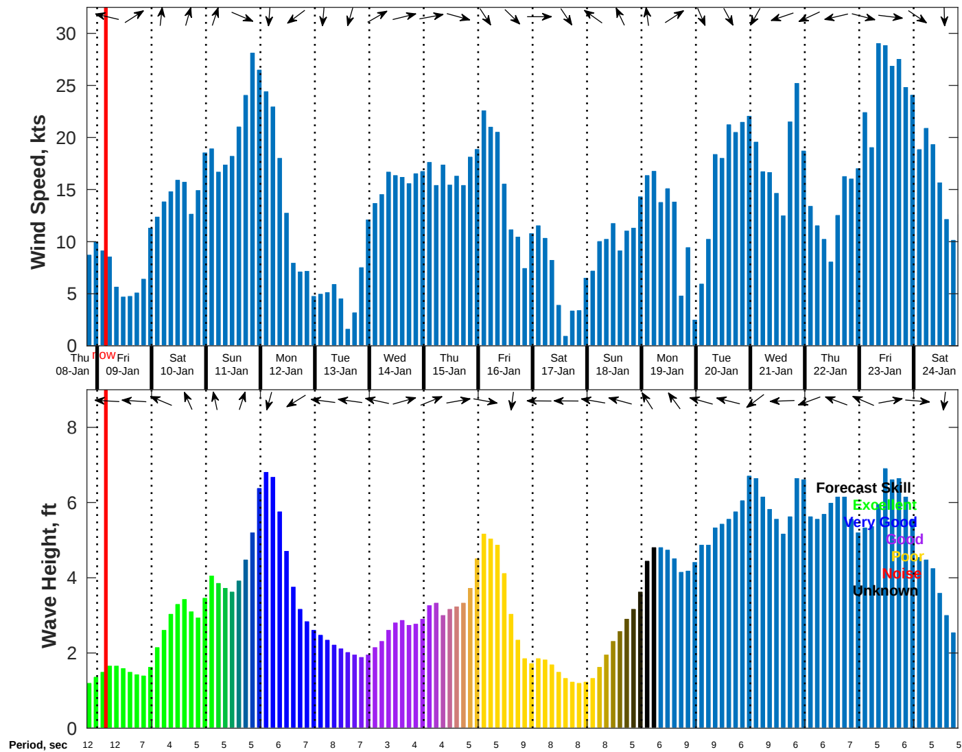
Wind & Wave Forecast for NDBC 41004 from 08-Jan-2026 19:00:00 to 24-Jan-2026 19:00:00
