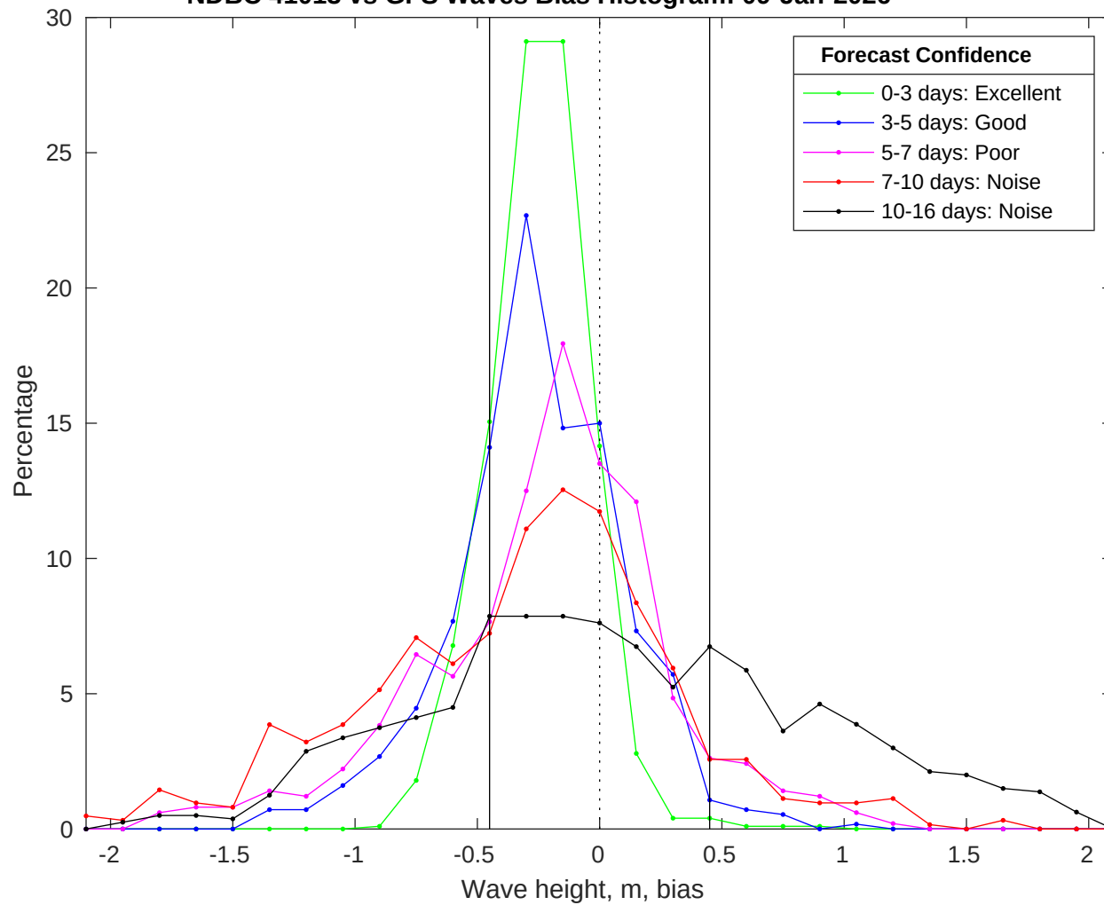
NDBC 41013 vs GFS Waves Bias Histogram: 09-Jan-2026
