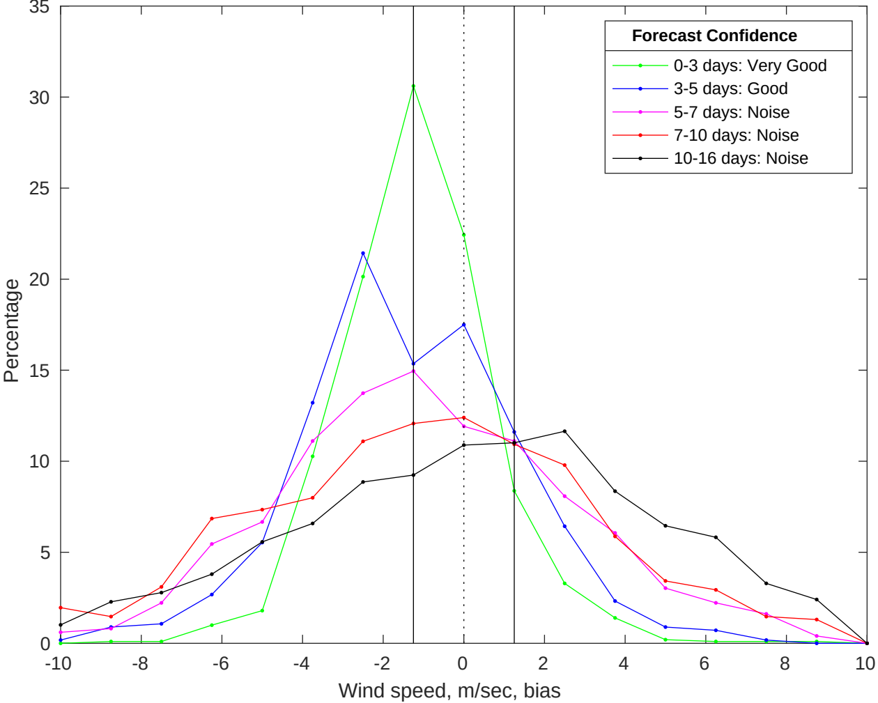
NDBC 41013 vs GFS Winds Bias Histogram: 09-Jan-2026
