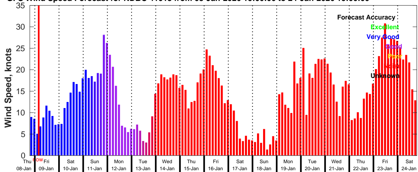
GFS Wind Speed Forecast for NDBC 41013 from 08-Jan-2026 19:00:00 to 24-Jan-2026 19:00:00
