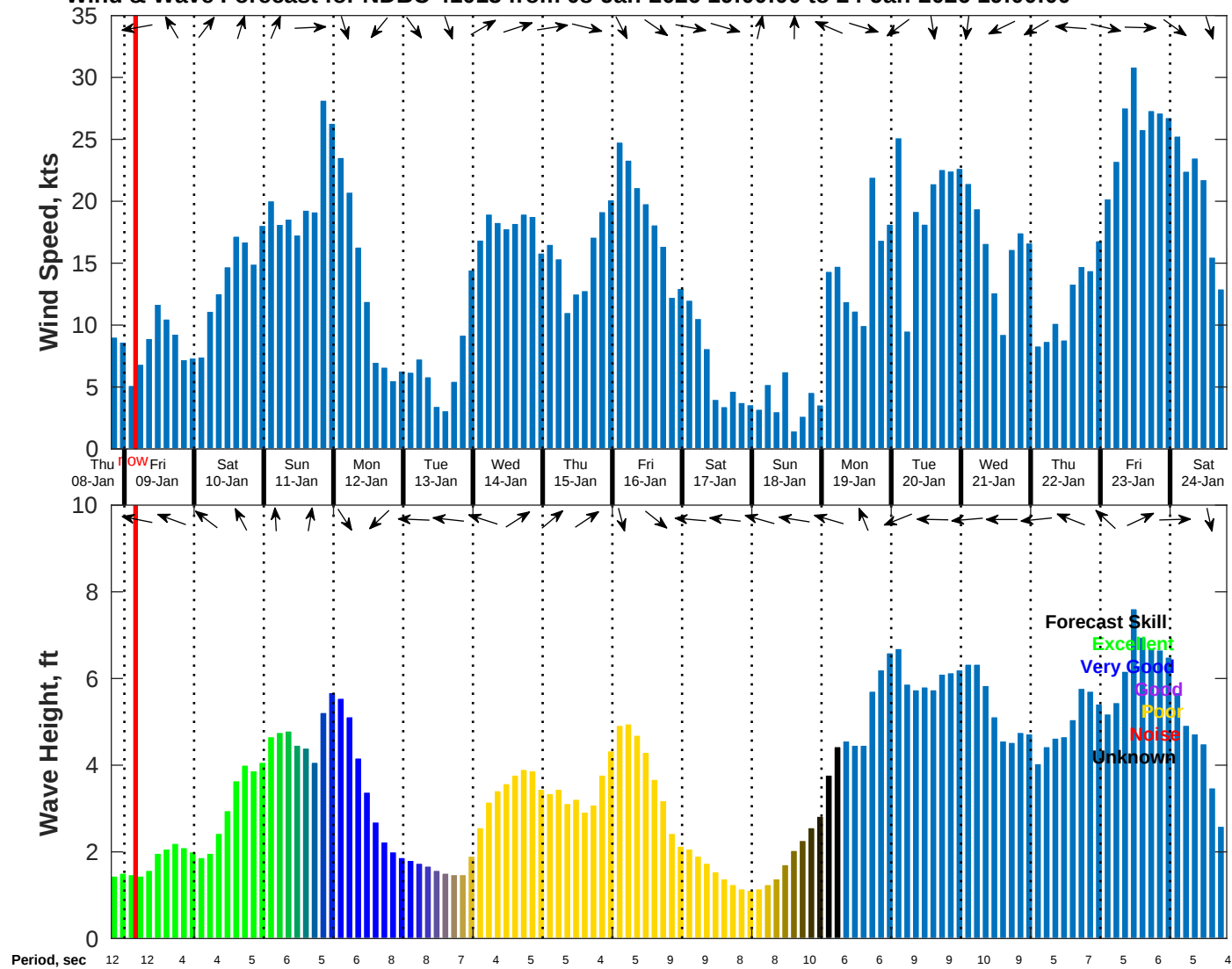
Wind & Wave Forecast for NDBC 41013 from 08-Jan-2026 19:00:00 to 24-Jan-2026 19:00:00
