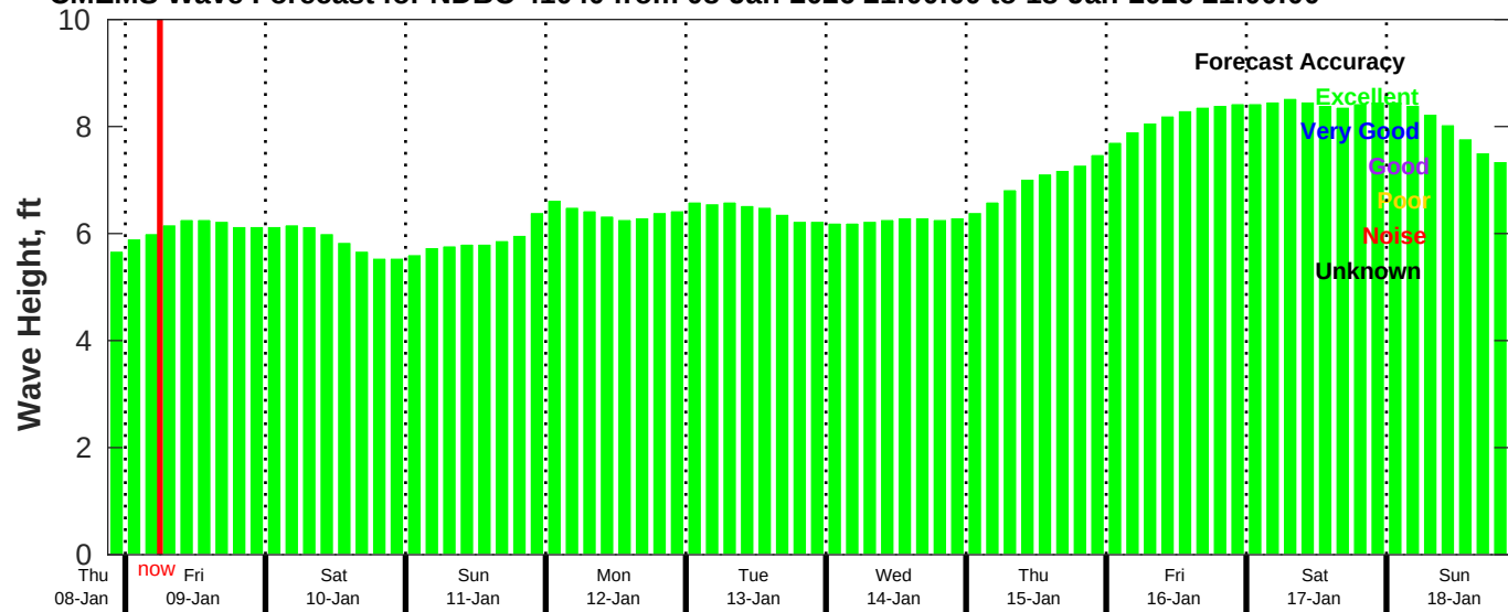
CMEMS Wave Forecast for NDBC 41040 from 08-Jan-2026 21:00:00 to 18-Jan-2026 21:00:00
