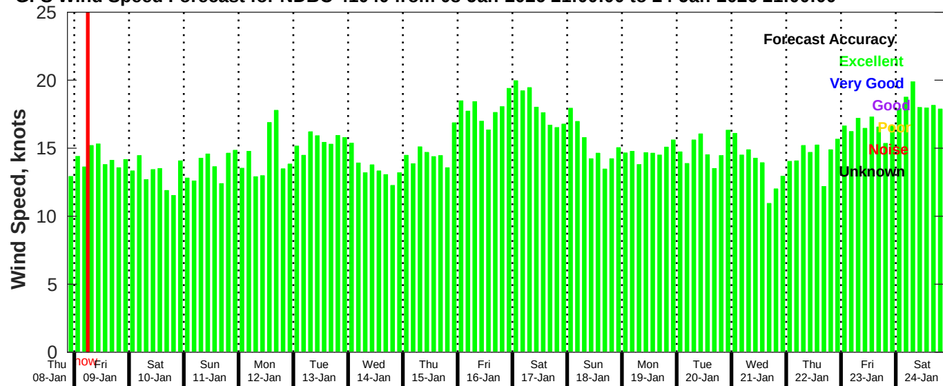
GFS Wind Speed Forecast for NDBC 41040 from 08-Jan-2026 21:00:00 to 24-Jan-2026 21:00:00
