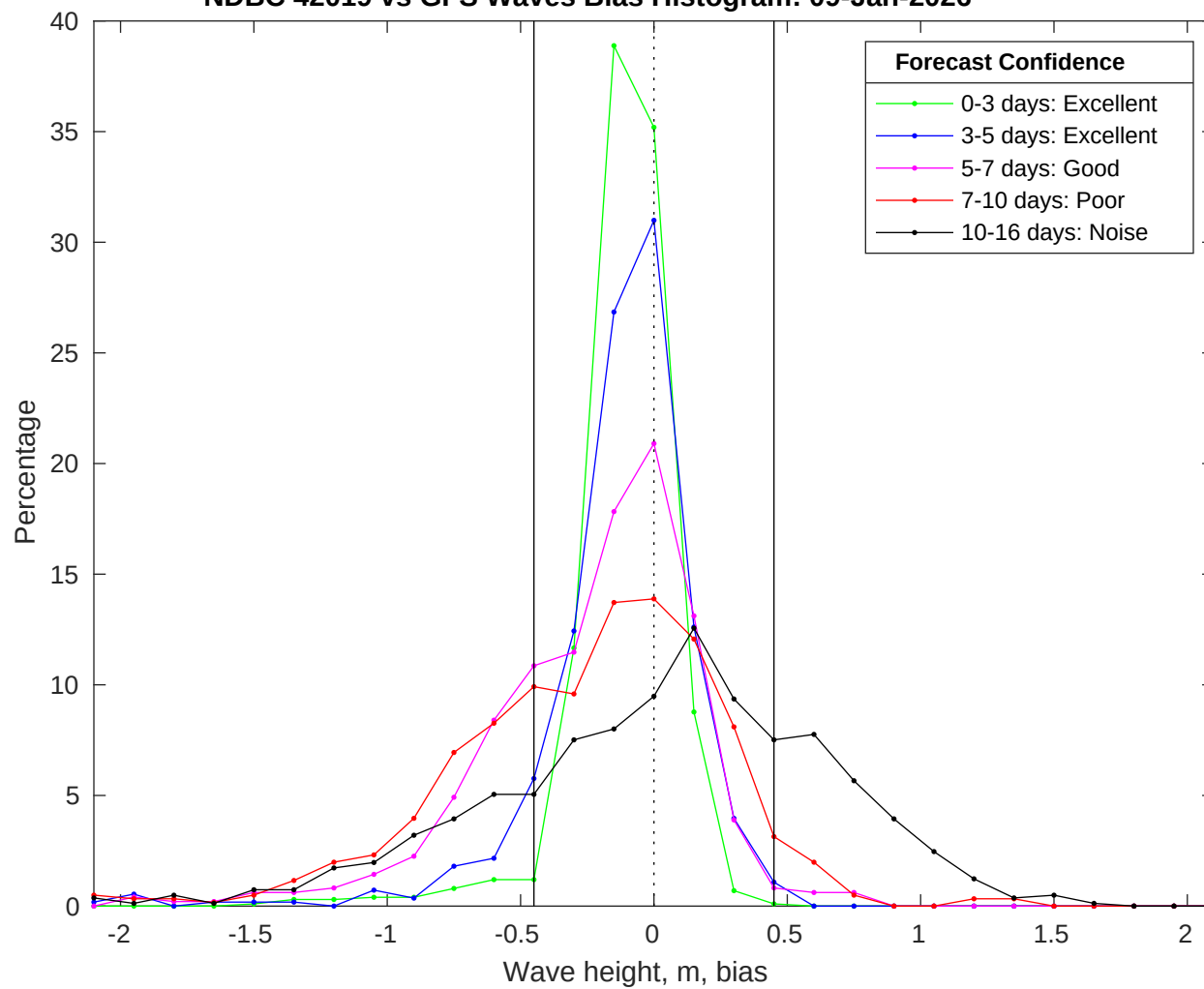
NDBC 42019 vs GFS Waves Bias Histogram: 09-Jan-2026
