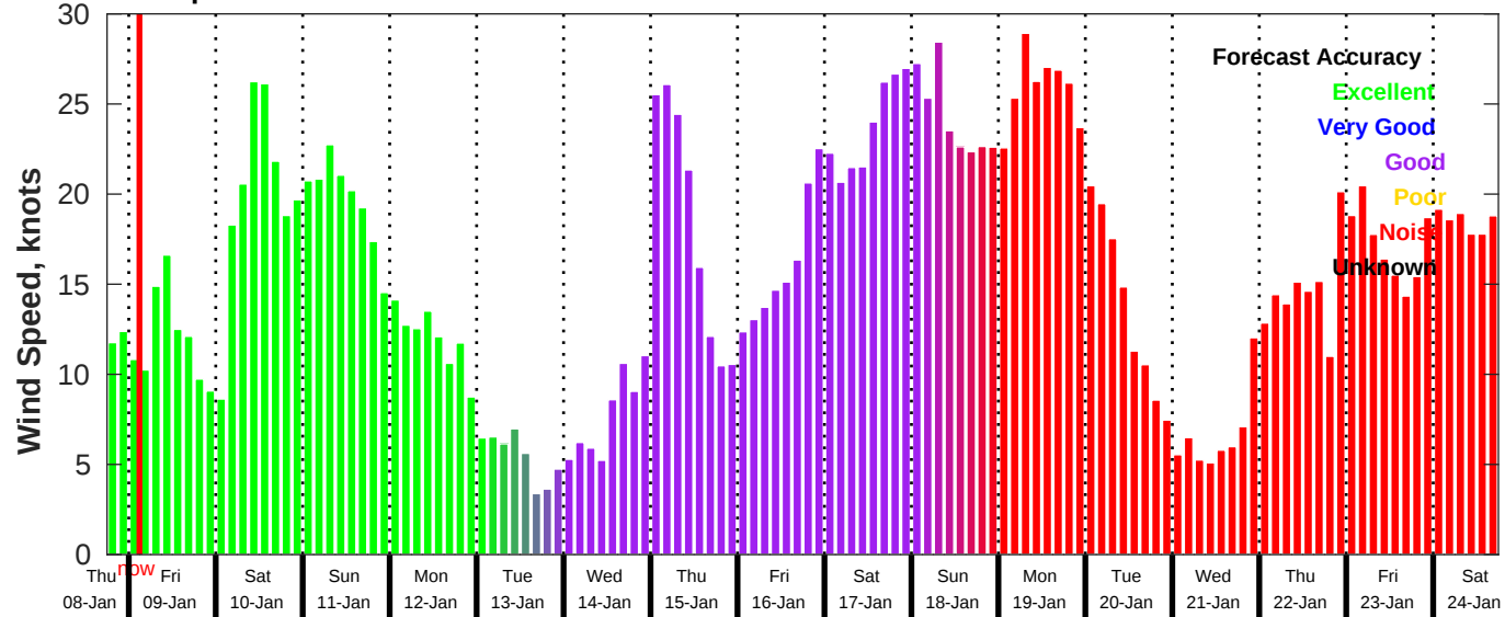
GFS Wind Speed Forecast for NDBC 42019 from 08-Jan-2026 18:00:00 to 24-Jan-2026 18:00:00
