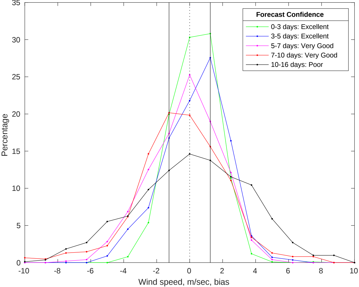
NDBC 42020 vs GFS Winds Bias Histogram: 09-Jan-2026
