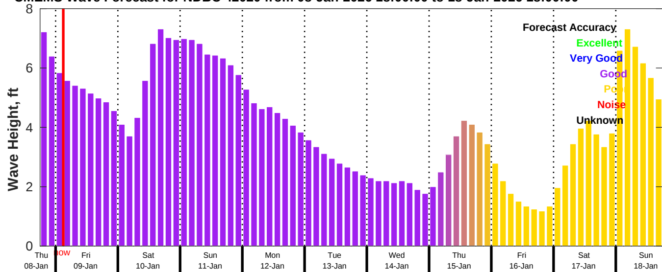
CMEMS Wave Forecast for NDBC 42020 from 08-Jan-2026 18:00:00 to 18-Jan-2026 18:00:00
