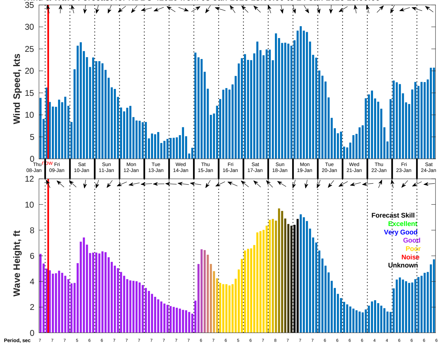
Wind & Wave Forecast for NDBC 42020 from 08-Jan-2026 18:00:00 to 24-Jan-2026 18:00:00
