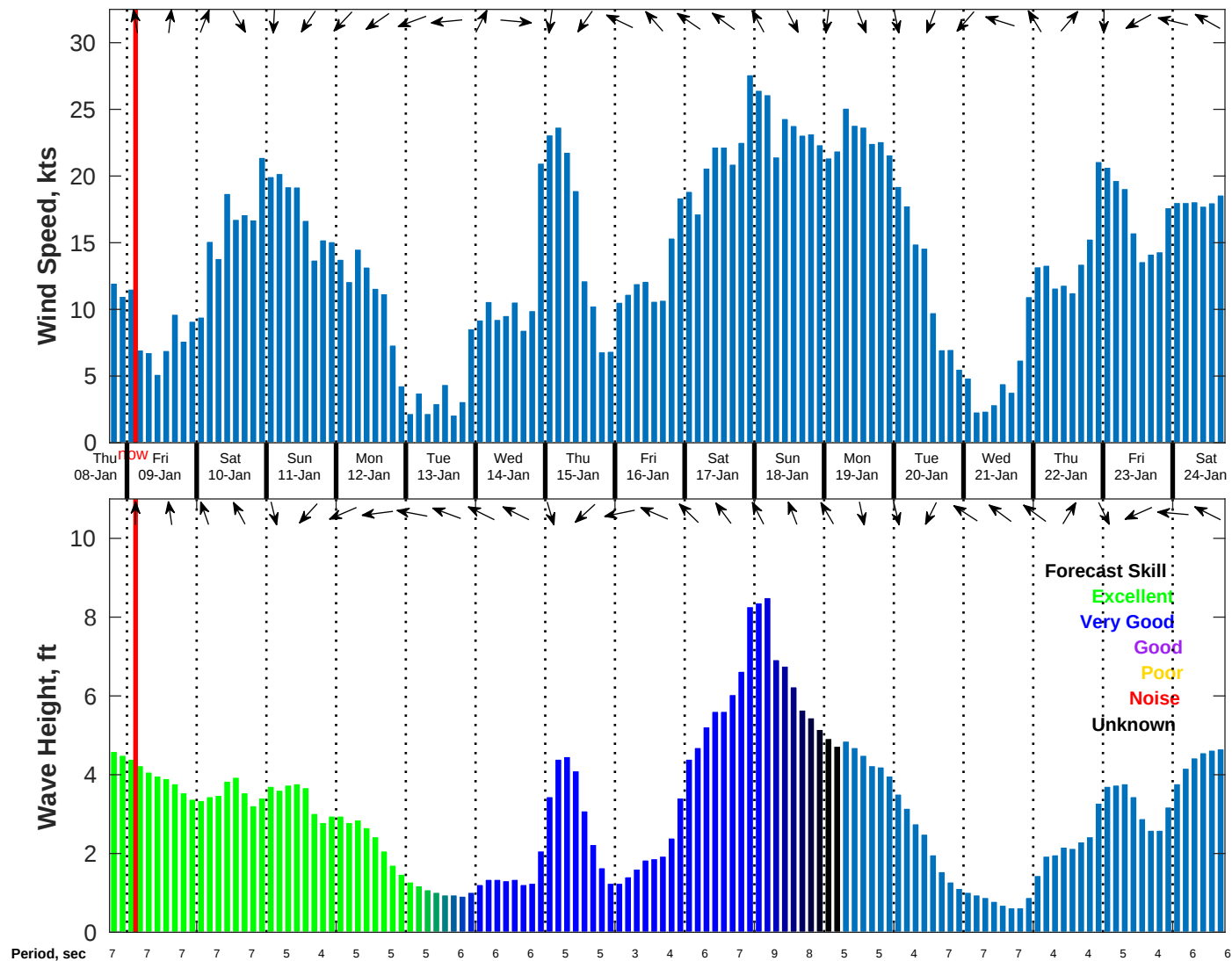
Wind & Wave Forecast for NDBC 42035 from 08-Jan-2026 18:00:00 to 24-Jan-2026 18:00:00
