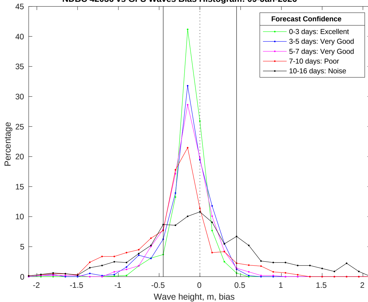
NDBC 42036 vs GFS Waves Bias Histogram: 09-Jan-2026
