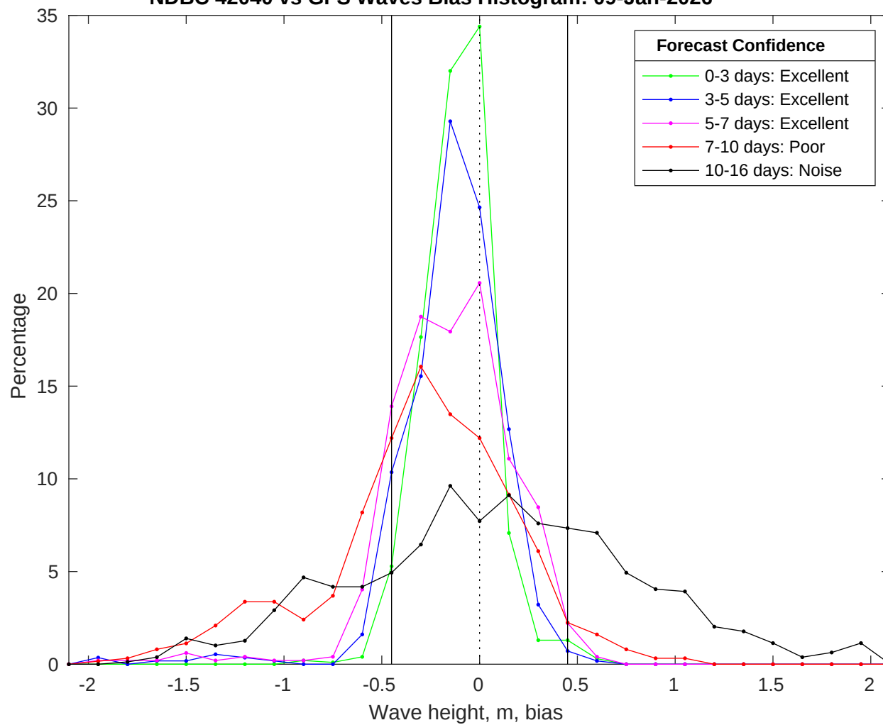
NDBC 42040 vs GFS Waves Bias Histogram: 09-Jan-2026
