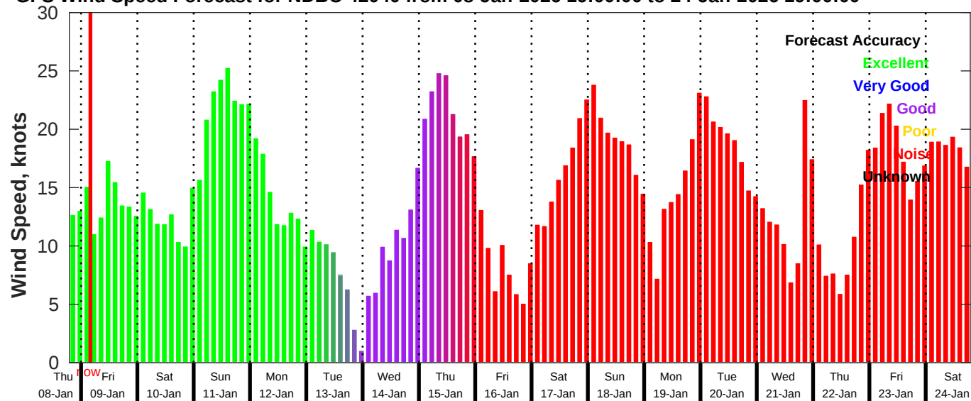
GFS Wind Speed Forecast for NDBC 42040 from 08-Jan-2026 19:00:00 to 24-Jan-2026 19:00:00
