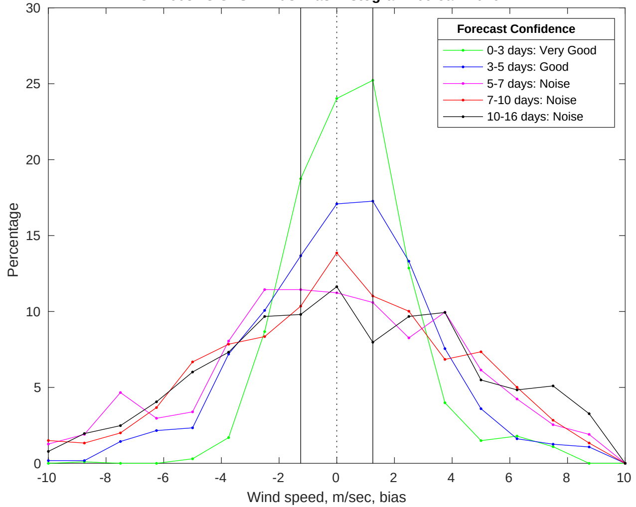
NDBC 44008 vs GFS Winds Bias Histogram: 09-Jan-2026
