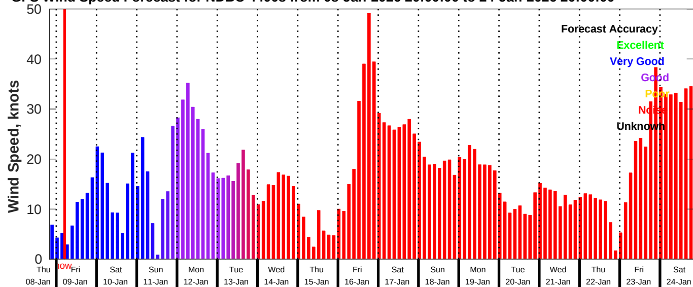
GFS Wind Speed Forecast for NDBC 44008 from 08-Jan-2026 20:00:00 to 24-Jan-2026 20:00:00
