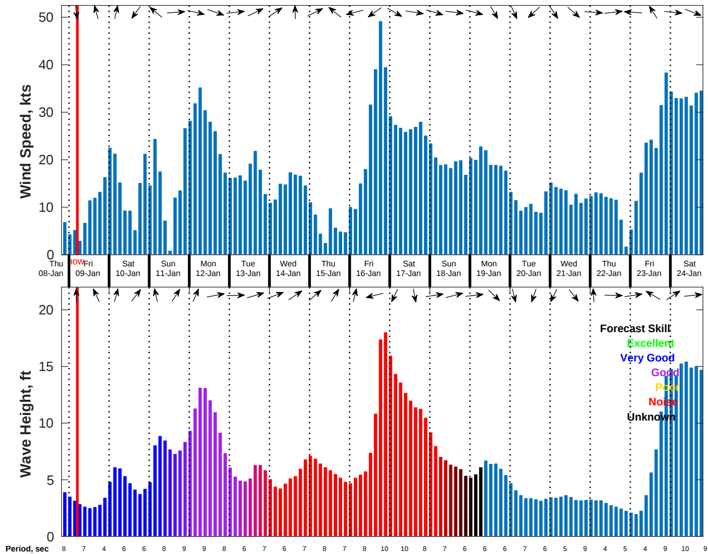
Wind & Wave Forecast for NDBC 44008 from 08-Jan-2026 20:00:00 to 24-Jan-2026 20:00:00
