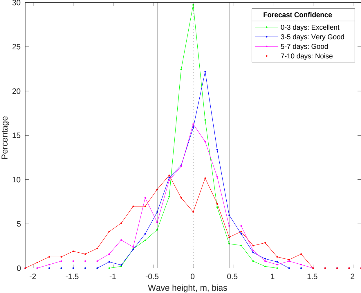
NDBC 46011 vs CMEMS Waves Bias Histogram: 09-Jan-2026
