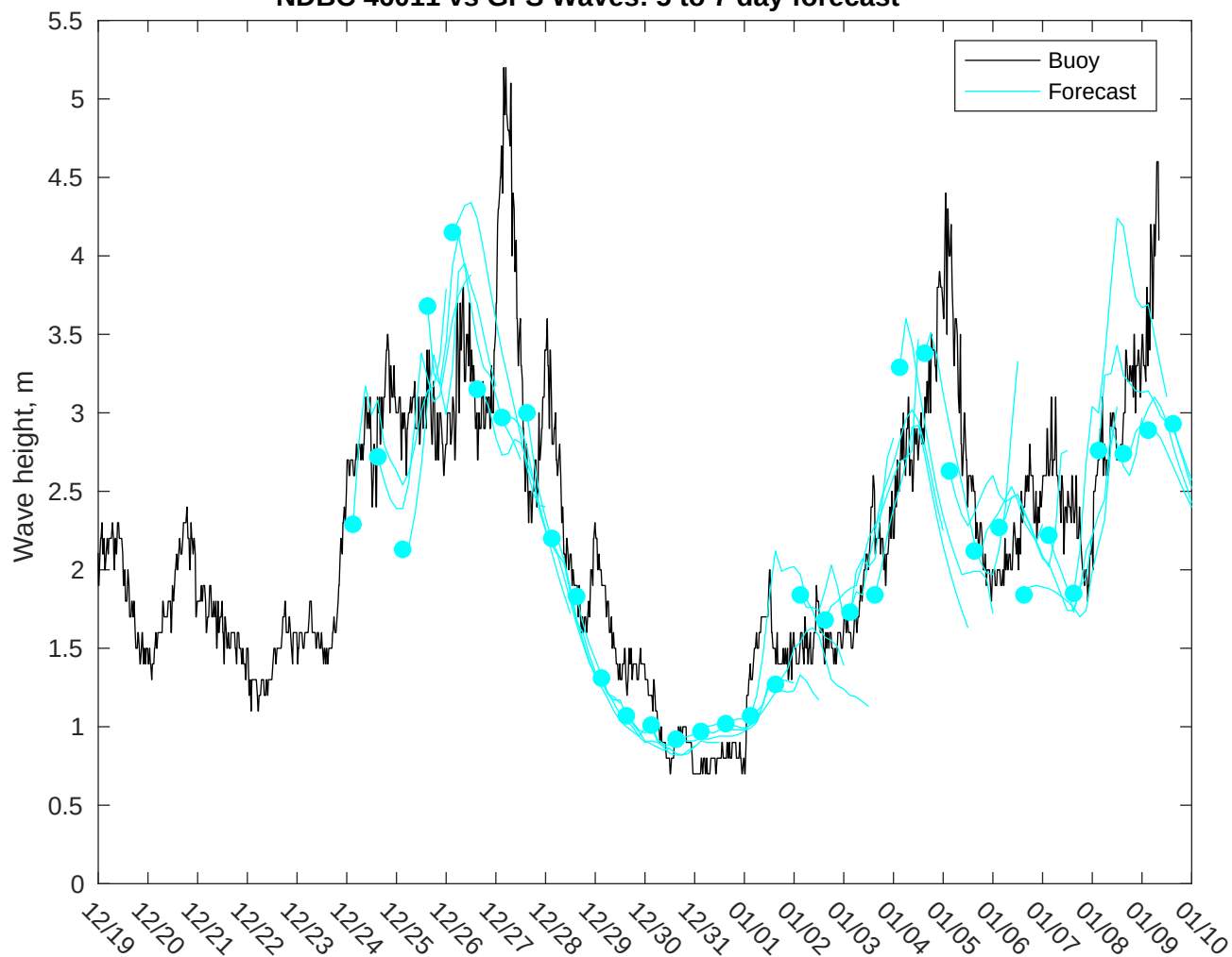
NDBC 46011 vs GFS Waves: 5 to 7 day forecast
