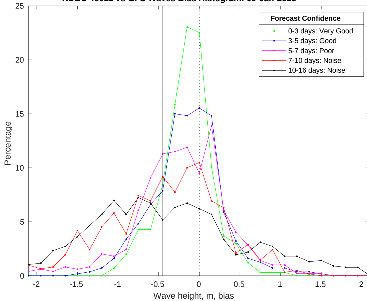
NDBC 46011 vs GFS Waves Bias Histogram: 09-Jan-2026
