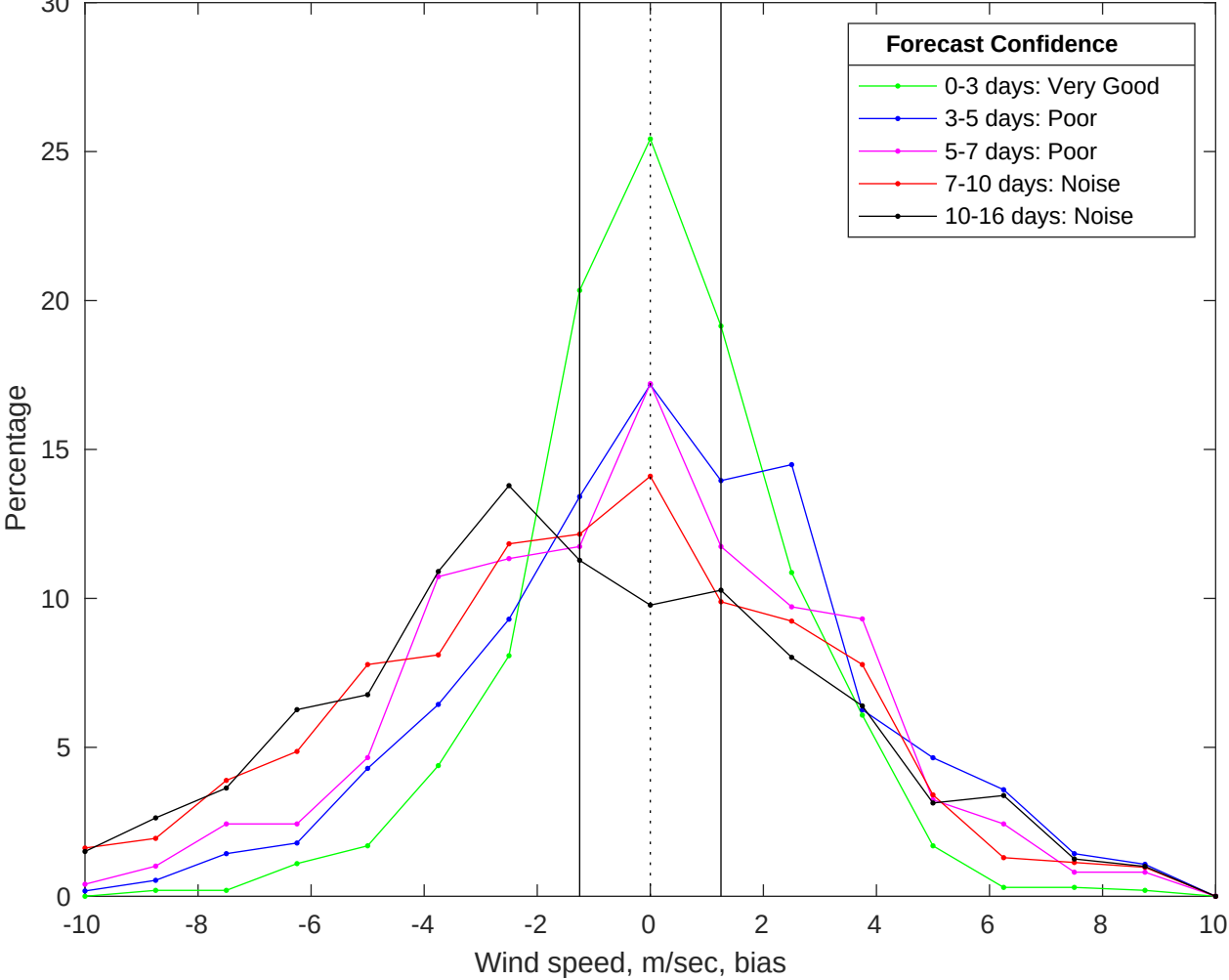
NDBC 46011 vs GFS Winds Bias Histogram: 09-Jan-2026
