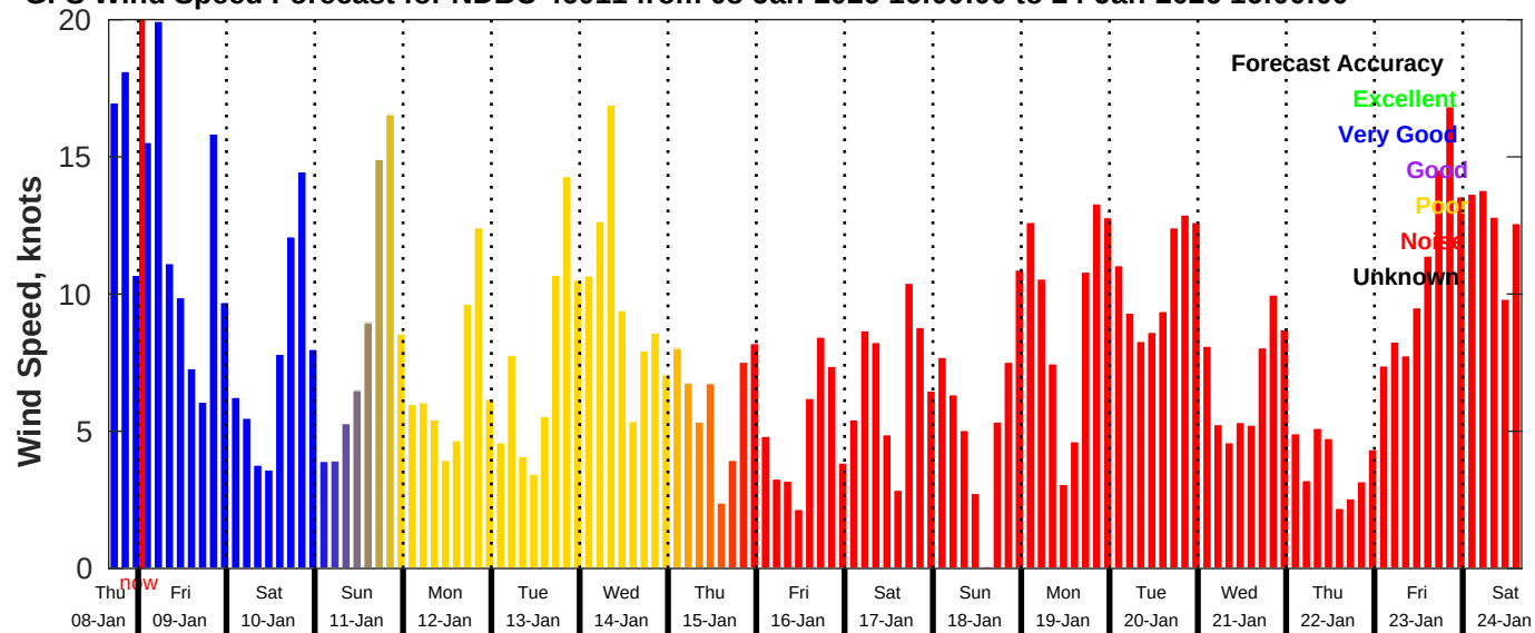
GFS Wind Speed Forecast for NDBC 46011 from 08-Jan-2026 16:00:00 to 24-Jan-2026 16:00:00
