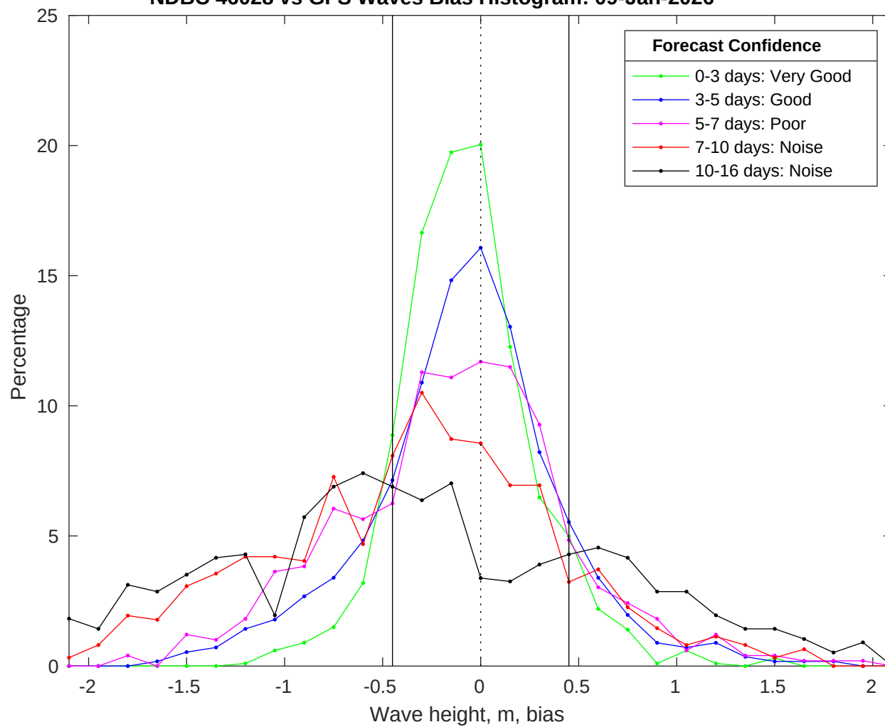
NDBC 46028 vs GFS Waves Bias Histogram: 09-Jan-2026
