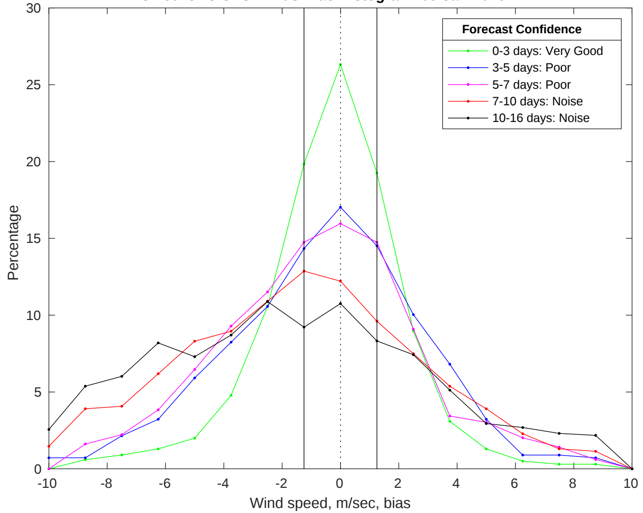
NDBC 46028 vs GFS Winds Bias Histogram: 09-Jan-2026
